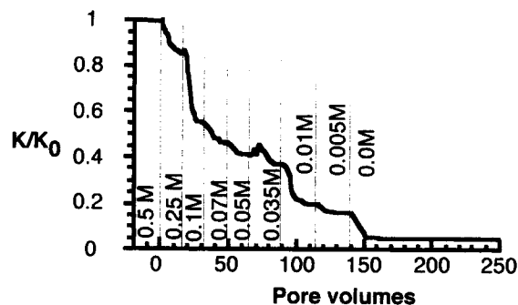
Figure 4. Permeability response of Stevens sandstone to step reduction in NaCl concentration.
