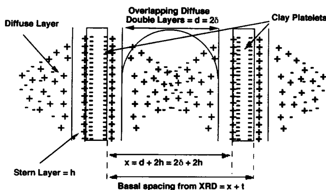
Figure 10. Model system of clay interaction.
