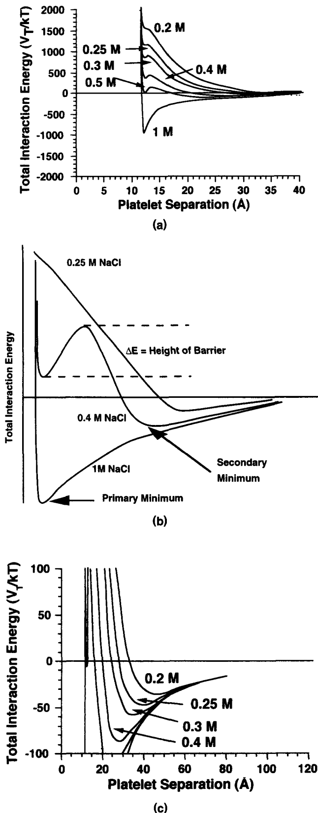
Figure 12. (a) Variation in primary minimum with salt concentration; (b) transition from primary minimum to secondary minimum; (c) variation in secondary minimum with salt concentration.
